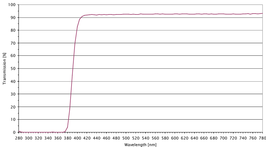
Spectral transmittance PLEXIGLAS® Film 0F008, thickness = 53 µm
